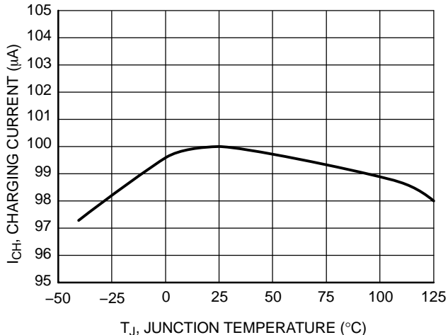
Figure 20. Charging Current vs. Temperature
